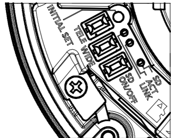
Detail B (2:1)
